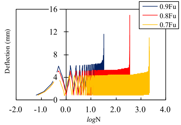
Figure 12: Deflection changes of flexural specimens under cyclic loading.
