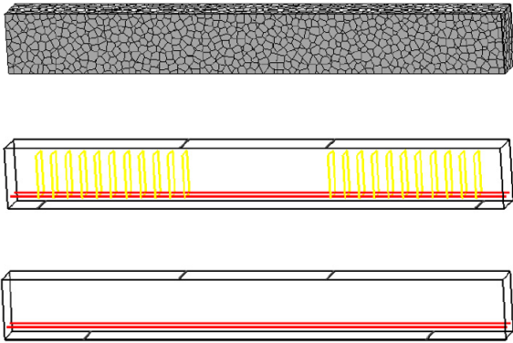
Figure 9: Outline of analytical mesh (upper) and rebar arrangements (middle: flexural specimen, lower: shear specimen).
