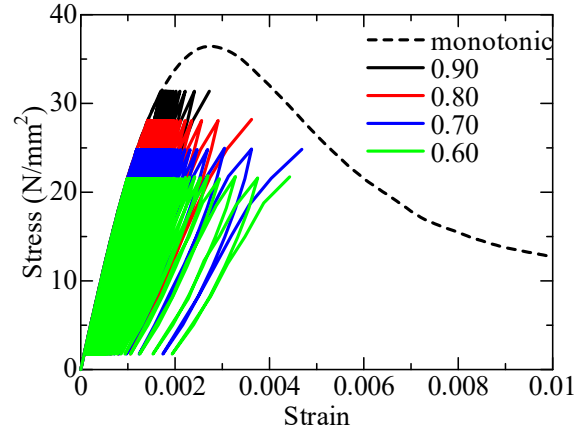
Figure 6: Stress-strain relationships of cylinder specimens.
