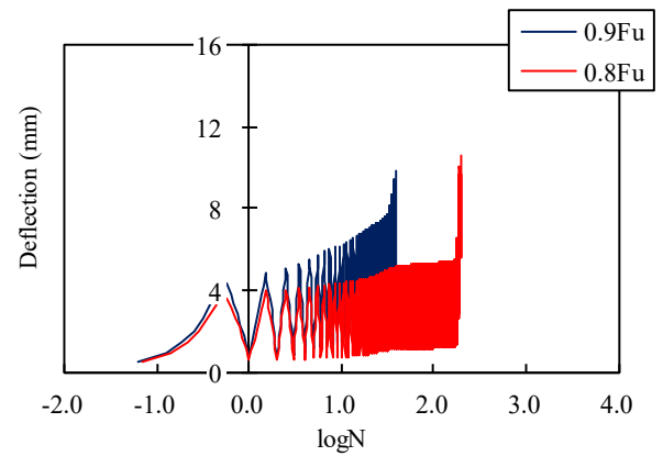
Figure 13: Deflection changes of shear specimens under cyclic loading.
