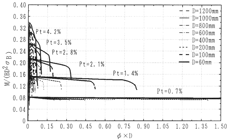
Fig.3 Normalized bending moment-normalized curvature curves
