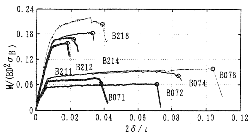
Fig.8 Normalized bending moment-displacement curves
