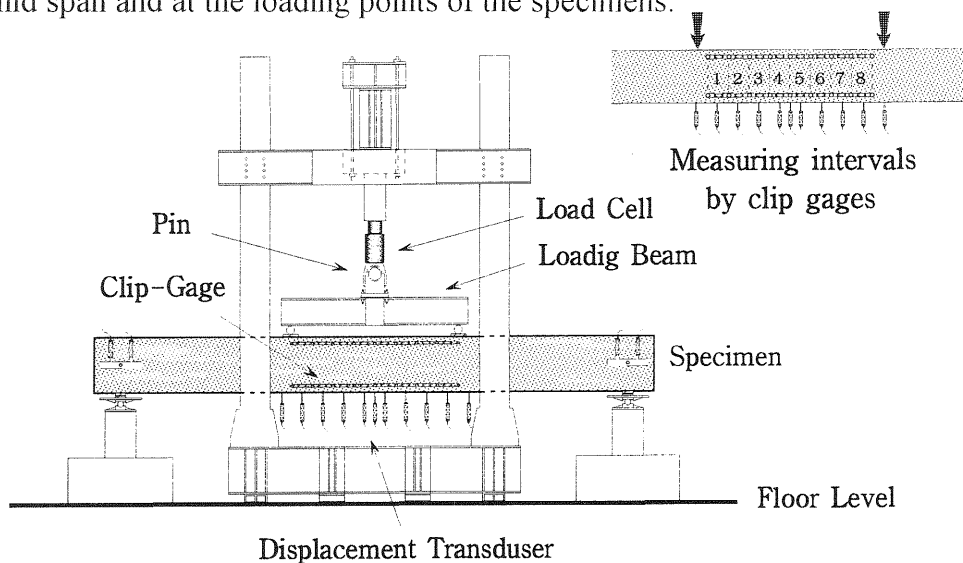
Fig.6 Loading setup and measurement system
