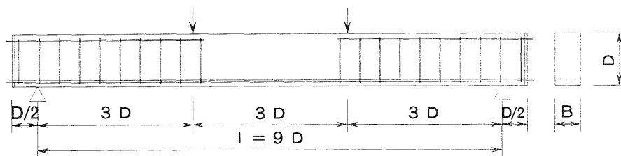
Fig.5 Configuration and bar arrangement of specimen
