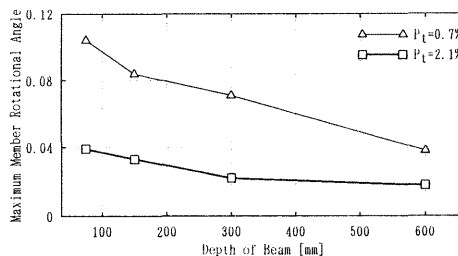
Fig.9 Maximum member rotational angle-depth relationship
