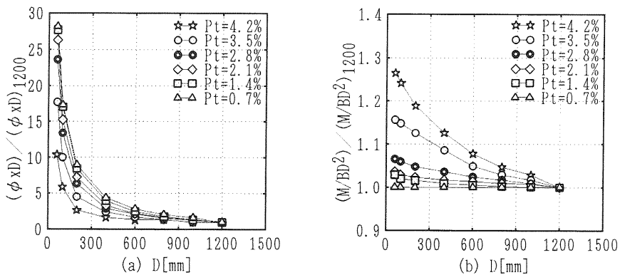
Fig.4 Normalized curvature-depth and bending moment-depth relationships
