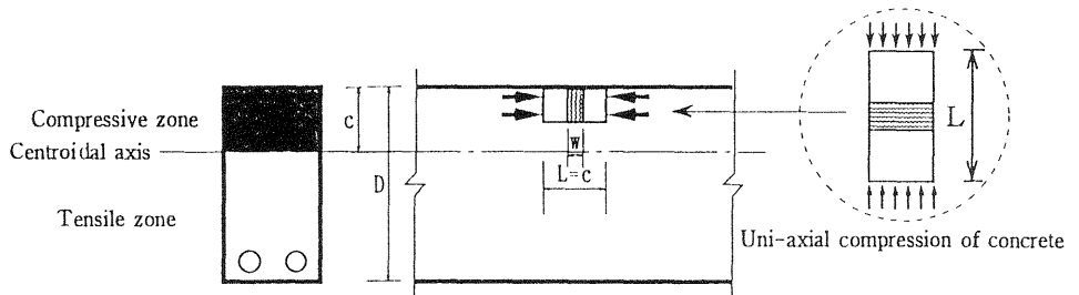
Fig.2 Concept of Compressive zone in RC beam
