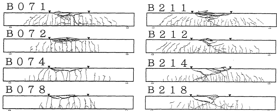
Fig.7 Failure Patterns of specimens
