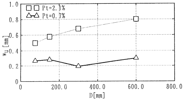
Fig.12 Relationship between best fit value of "Wu" and beam depth
