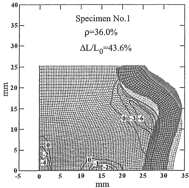
Figure 4. The experimental deformed shape of a typical specimen type no.1 and its prediction by the finite element analysis. Also shown are the contours of equal K_t \leq 0 normalized by Young's modulus E of concrete.
