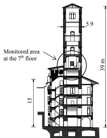
Figure 6. Tower cross section.
