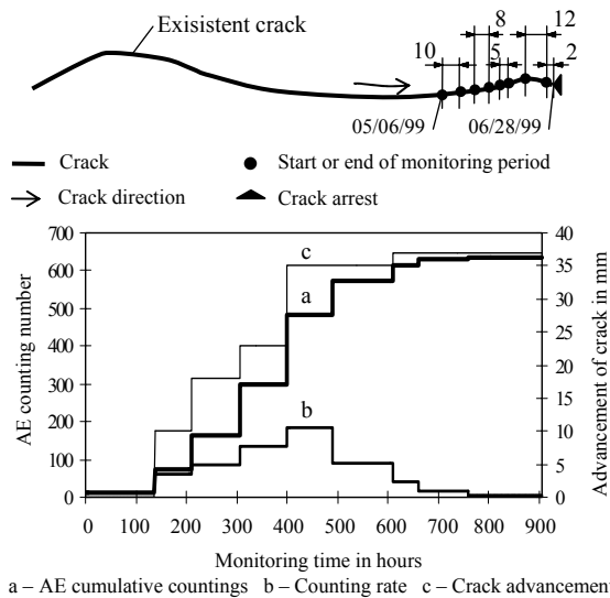
Figure 3. Crack n. 1. Development and AE monitoring results.
