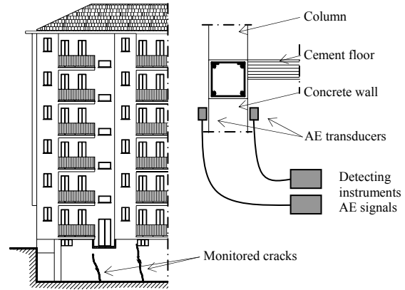
Figure 9. Building in Cascine Vica. Cracking framework and location of transducers on the concrete wall.
