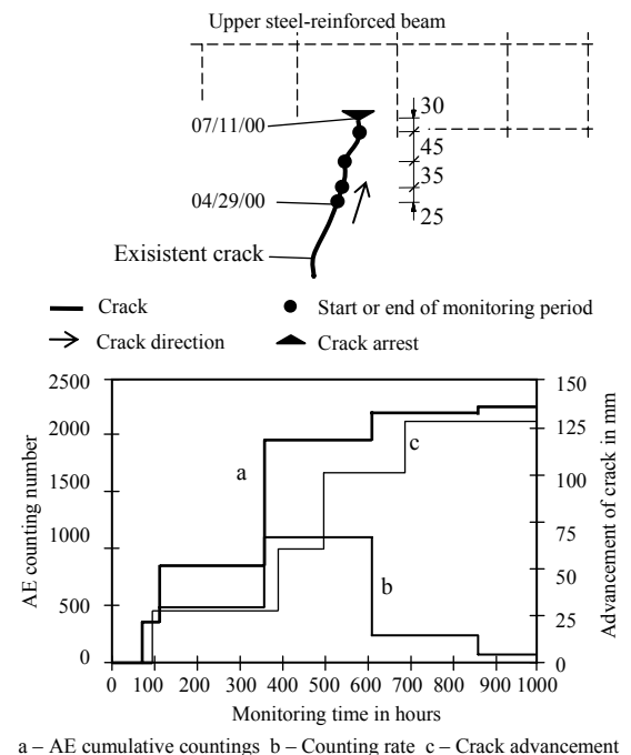
a – AE cumulative countings b – Counting rate c – Crack advancement Figure 10. Results of monitoring with AE technique.
