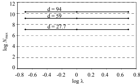
Figure 17. Shape-effect on N_{\max} .
