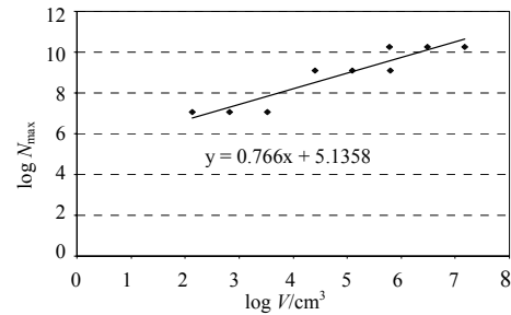
Figure 15. Volume-effect on N_{\max} .
