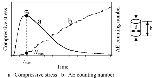
Figure 14. Stress and cumulated event number versus time.
