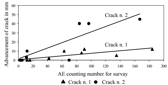
Figure 4. Diagrams of correlation between the number of AE events and the crack advancement.
