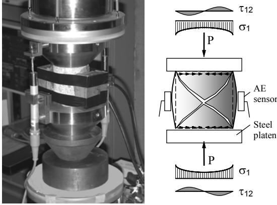
Figure 13. Apparatus adopted for compression tests.
