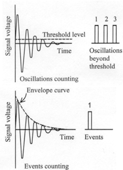
Figure 1. Detected signals by AE technique.
