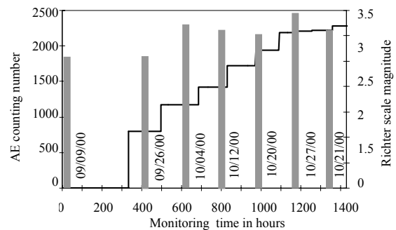
Figure 7. Sineo Tower monitoring.
