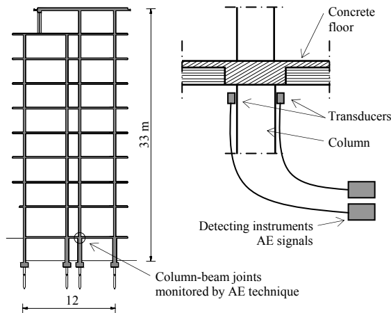
Figure 8. Building in Moncalieri. Structural section of the building and location of transducers on column-beam joints.
