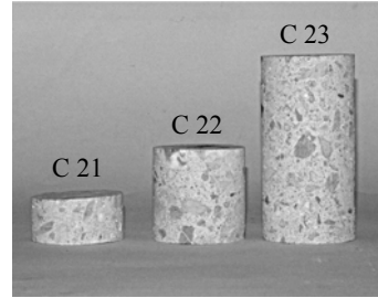
Figure 12. Geometries of some tested specimens.
