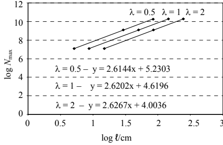
Figure 16. Linear size-effect on N_{\max} .
