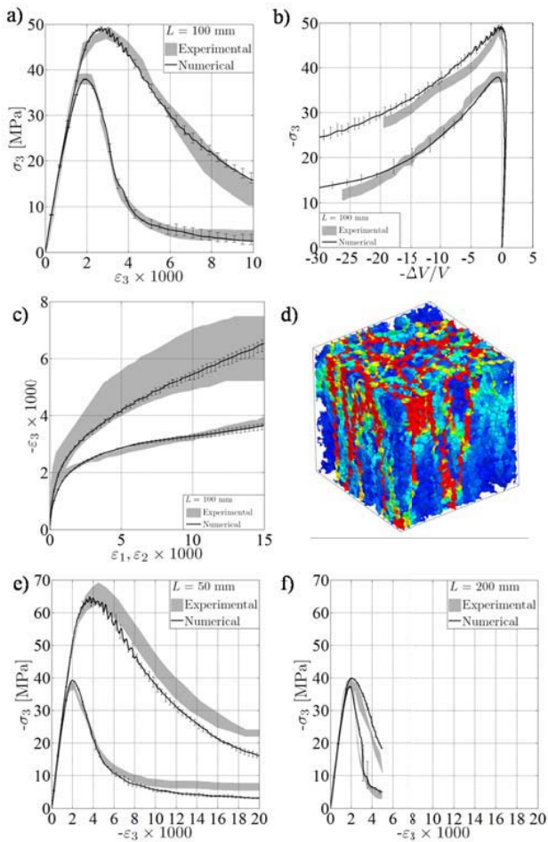
Figure 3: Uniaxial compression test results.
