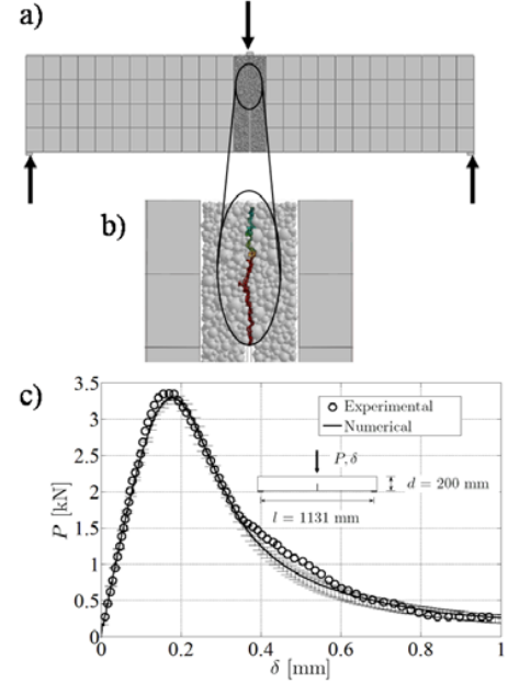
Figure 2: Three-point bending tests.
