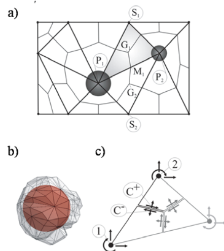
Figure 1: a) Meso-structure tessellation. b) Three-dimensional discrete particle. c) Definition of nodal degrees of freedom and contact facets in two-dimension.
