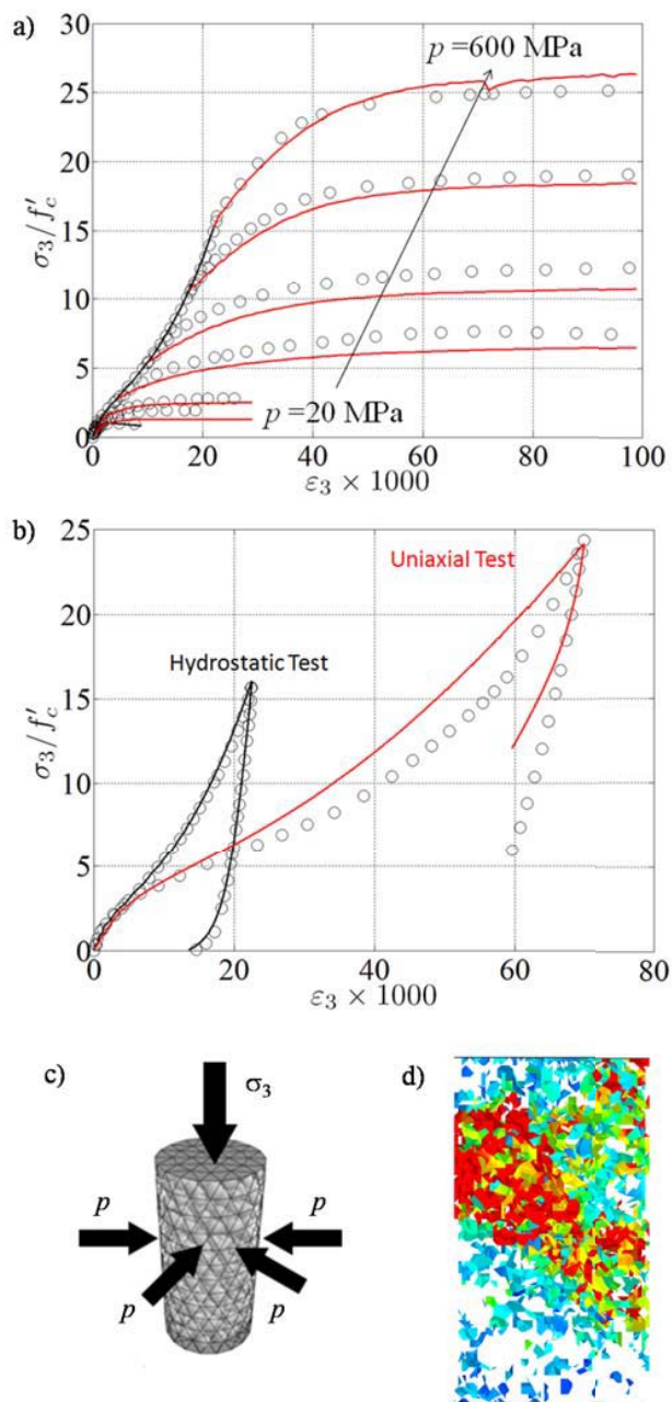
Figure 5: Triaxial test results.
