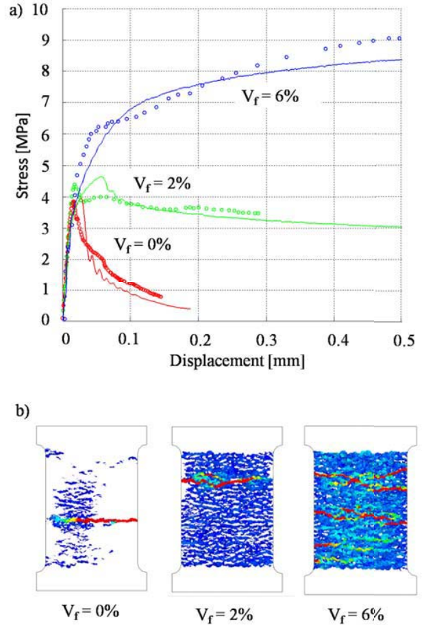
Figure 6: Simulation of fiber reinforced concrete.
