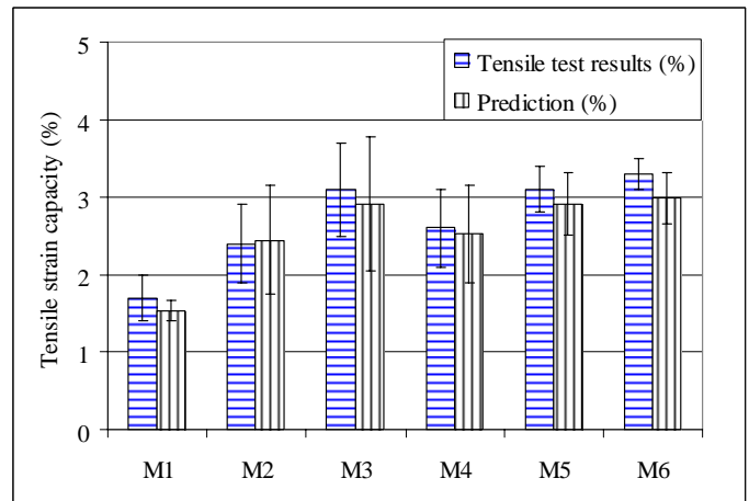
Figure 6. Comparison of tensile strain capacity from test and prediction (Zhou et al. 2009a).
