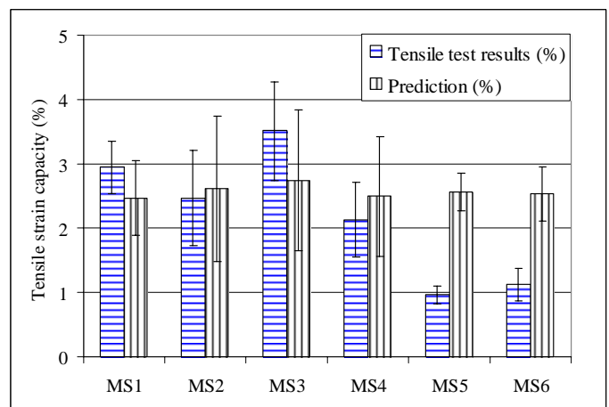
Figure 7. Comparison of tensile strain capacity from test and prediction (Zhou et al. 2009b).
