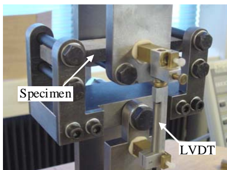
Figure 3. Four-point bending test set-up.
