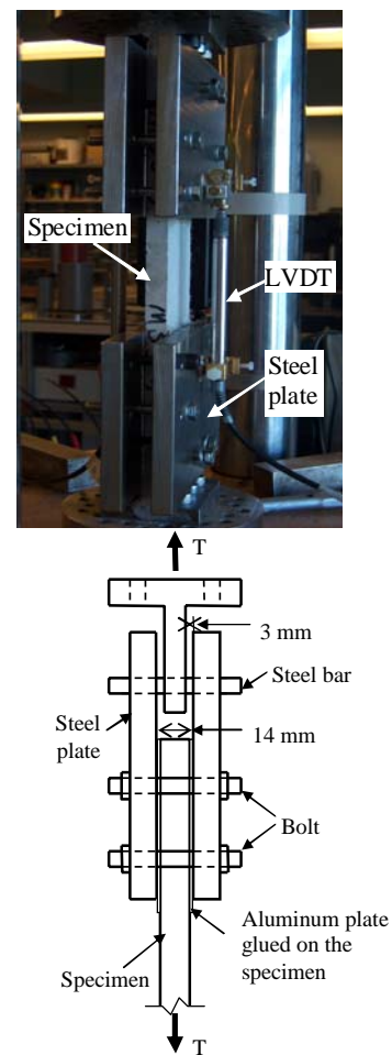
Figure 4. Uniaxial tensile test set-up.
