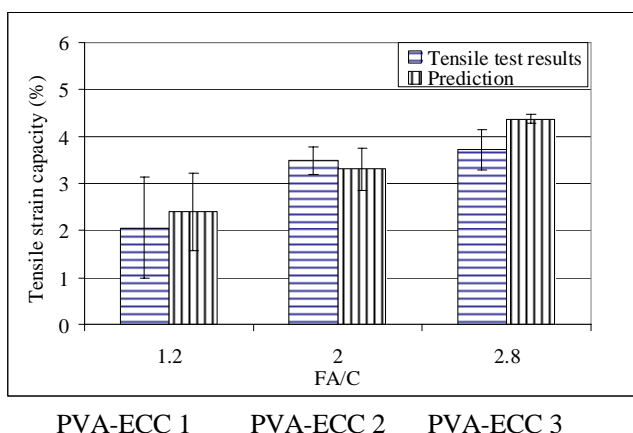
Figure 5. Comparison of tensile strain capacity from test and prediction.
