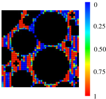
Figure 10. Damage field ( D_x variable) for the compression test.
